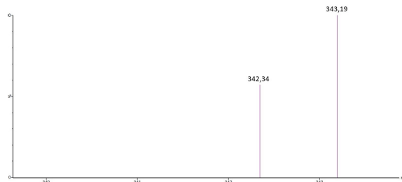
MS spectrum of LIB'UP® U-[13C22]-T2 Toxin.
