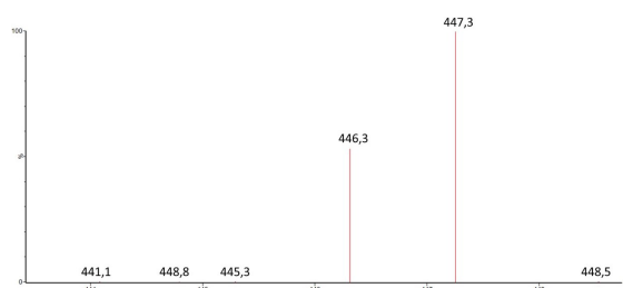
Spectre MS de l'étalon LIB'UP® U-[ 13 C22]-Toxine HT2
